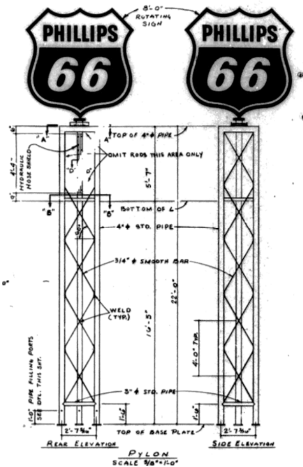
FIGURE 9: Original 1963 Signage Pylon Elevations
