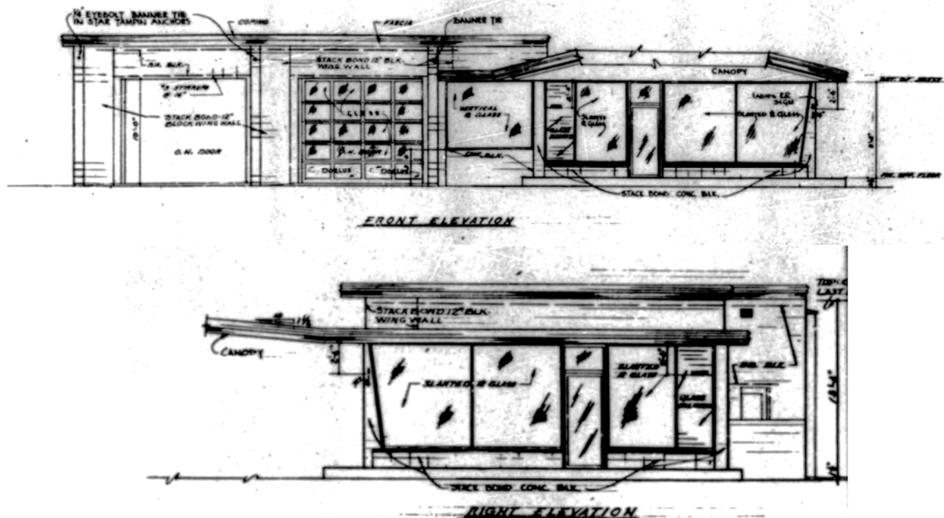
FIGURE 7: Original 1963 Elevations
